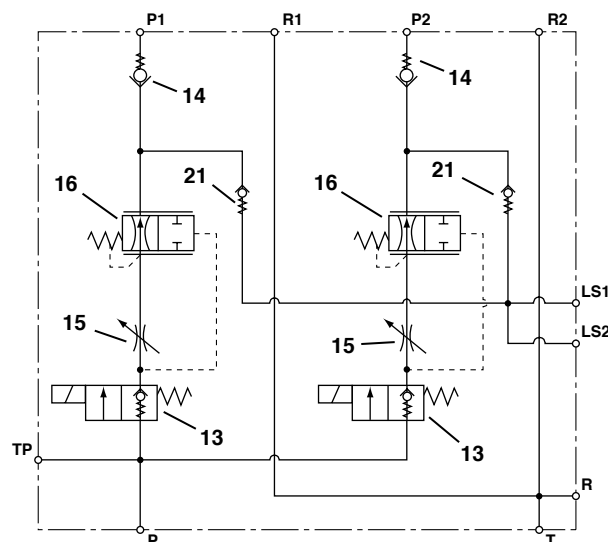
Hydraulic Schematic 3181640
