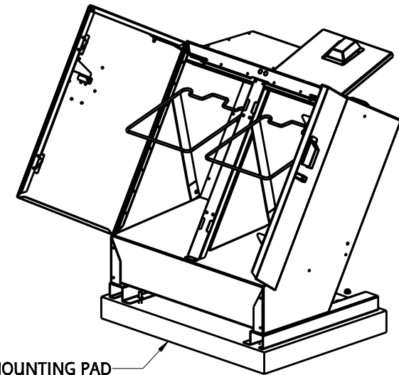
MOUNTING PAD (OPTIONAL)
